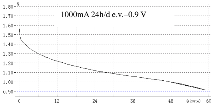
Chart 1. Discharge diagram
